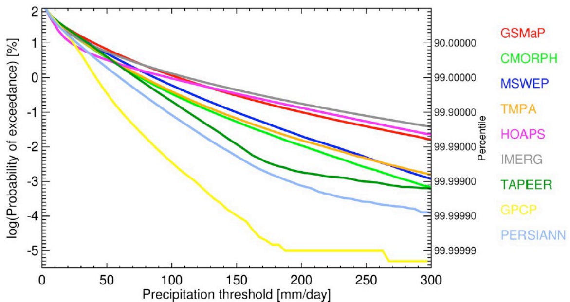
Figure 2.5.2. Probability of exceedance of daily 1^{\circ} \times 1^{\circ} accumulated precipitation over the tropical ocean ( 30^{\circ}\text{S} – 30^{\circ}\text{N} ) for the period 2017–2017 except for the TAPEER product where it is restricted to the 2012–2016 period.
