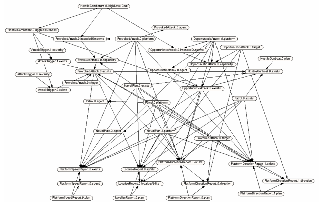
Figure 3: Situation-Specific Bayesian Network
