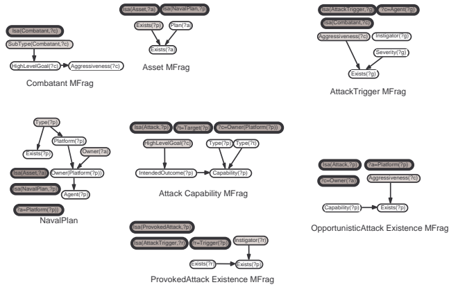
Figure 2: MFrag for Naval Attack MTheory
