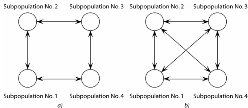
Figure 4. Investigated connectivity topologies a) ring, b) fully connected.
